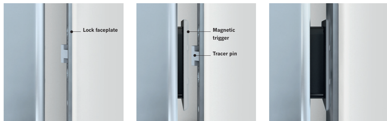
03 When you close a door that has the metallic faceplate ... the magnetic trigger is pulled in ... and the tracer pin retracts. This prevents it from striking against the door frame, thus avoiding scratches.
